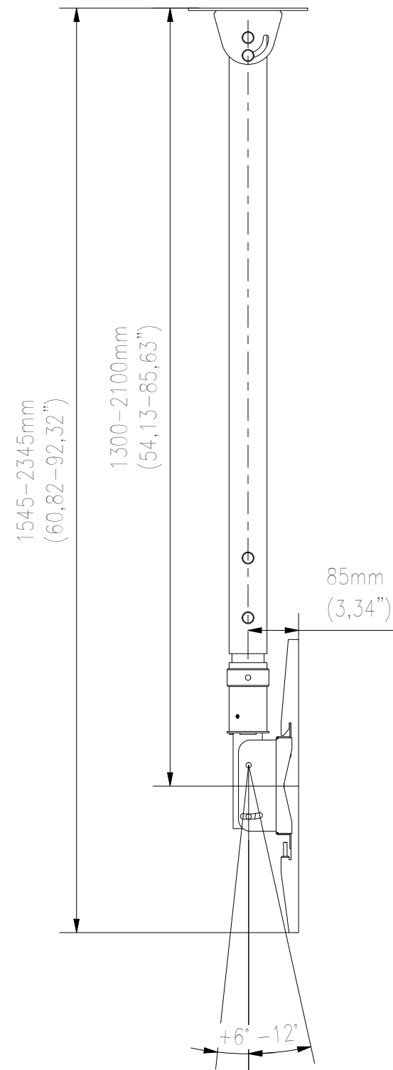
SIDE VIEW
