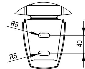
DETAIL G SCALE 1 : 5
