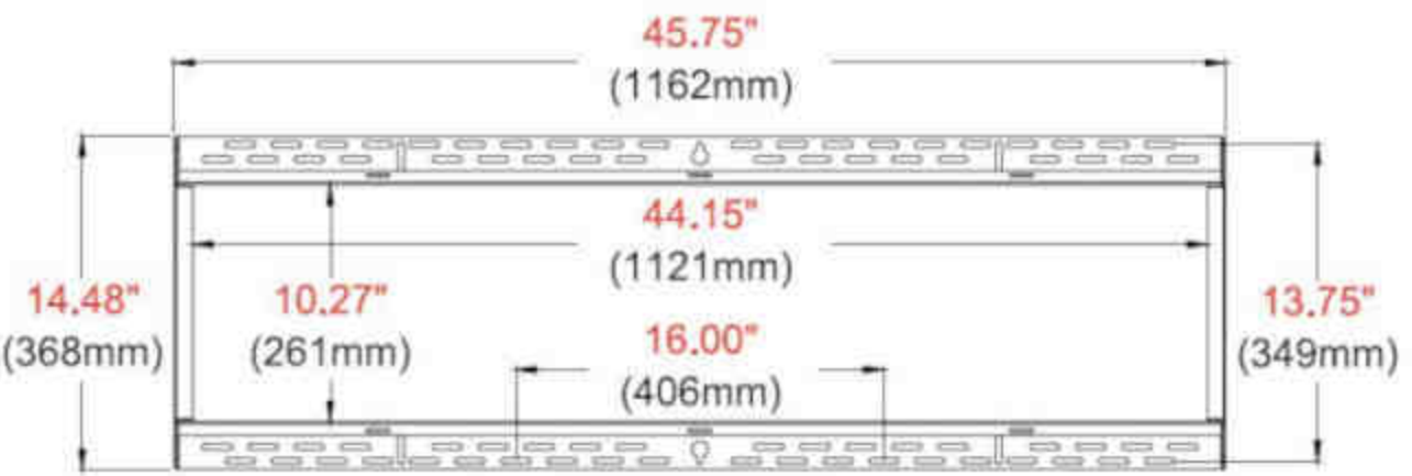
WALL PLATE DETAIL
