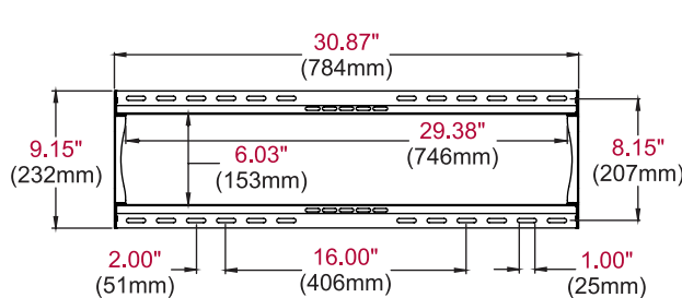
WALL PLATE
