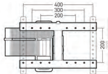
TILT AND SWIVEL WALL MOUNT WITH 538MM OFFSET FOR OLED TVs
