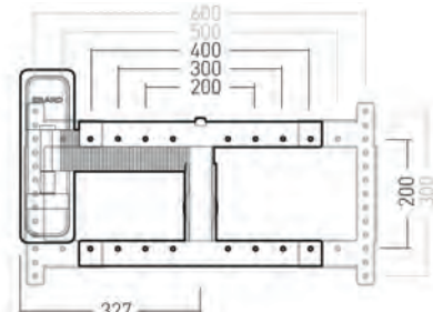
TILT AND SWIVEL WALL MOUNT WITH 325MM OFFSET 325MM FOR OLED SCREENS TVs
